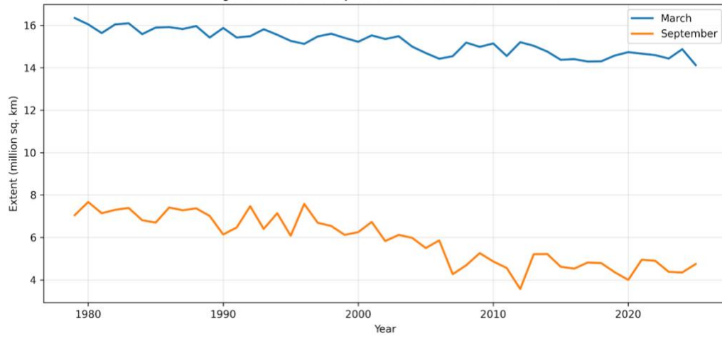
Figure 4. March vs September Sea Ice Extent Over Time
